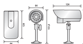
Night Vision Camera : SOC-N120
